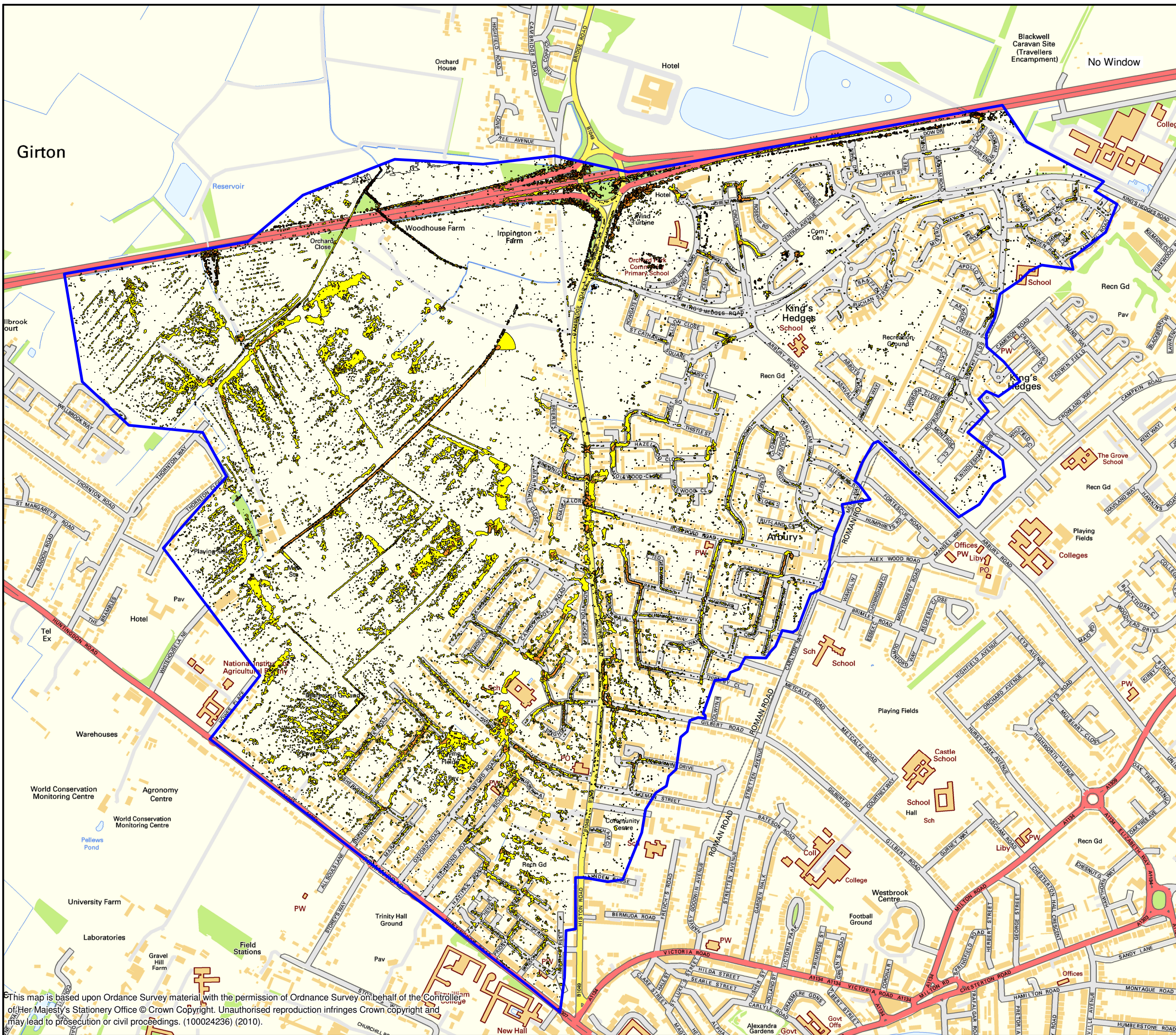
FIGURE F41 3.3% AEP "DO MINIMUM" PLUVIAL MODELLING MAXIMUM VELOCITY - KING'S HEDGES AND ARBURY
